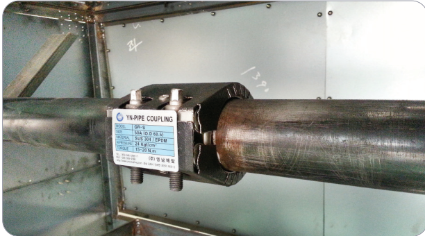
▲ The product just before the fire test, after being installed in a furnace
